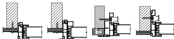
Vinyl with nail fin
