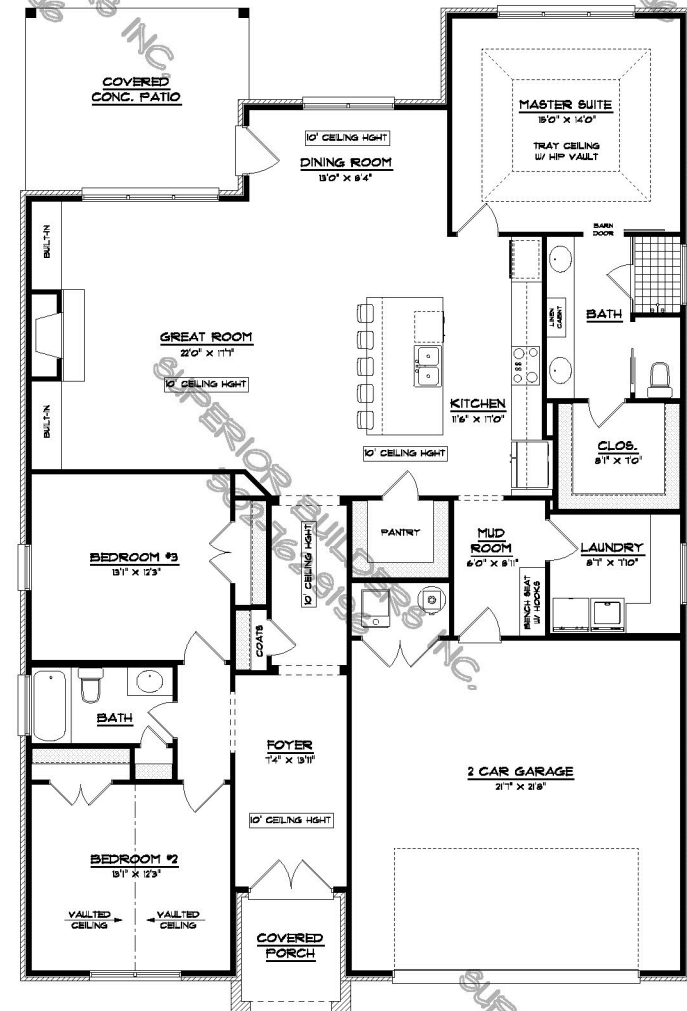
FLOOR PLAN
