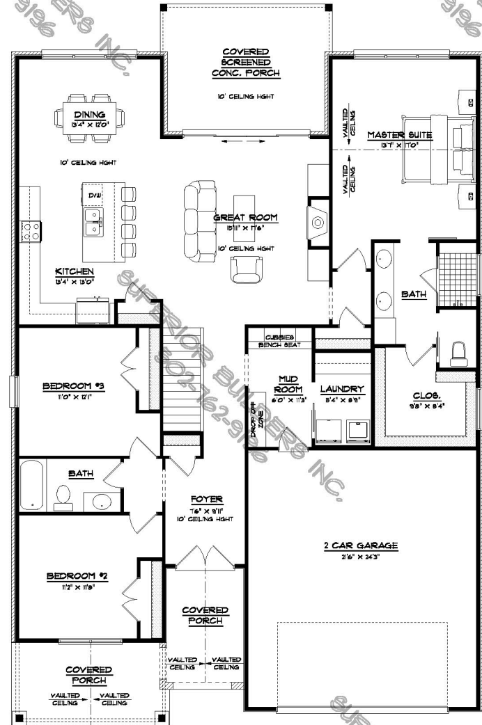
FLOOR PLAN
