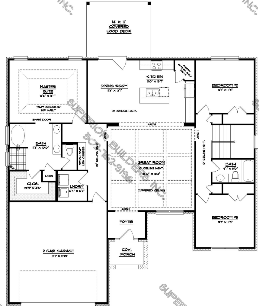
FLOOR PLAN 1,996 SQ. FT.
