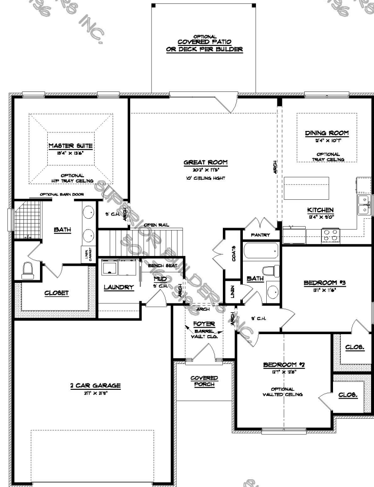
FLOOR PLANS B
