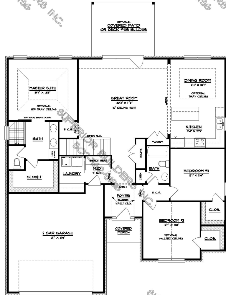
FLOOR PLAN A1
