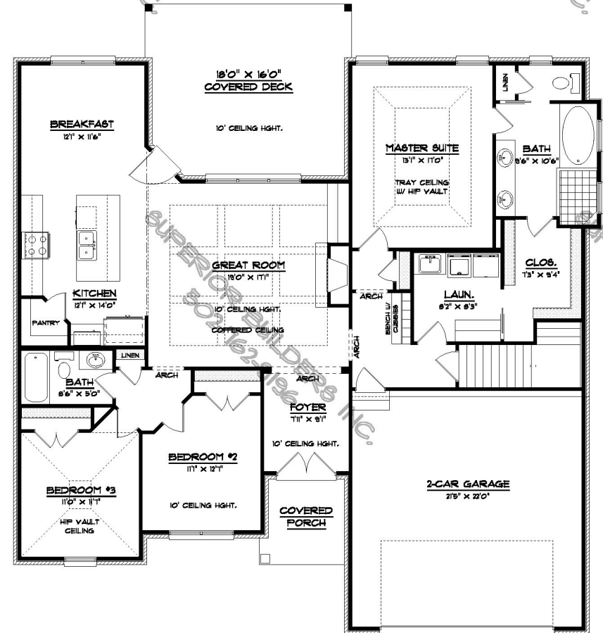
FLOOR PLAN
