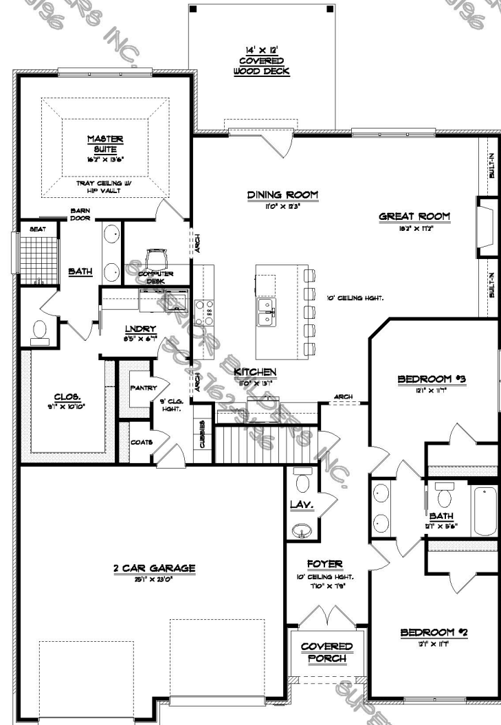
FLOOR PLAN 2,038 SQ. FT.
