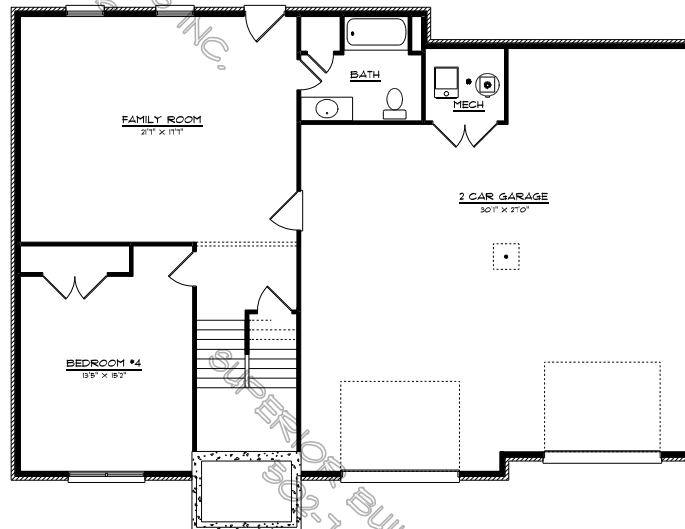
FOUNDATION PLAN 826 SQ.FT. FINISHED
